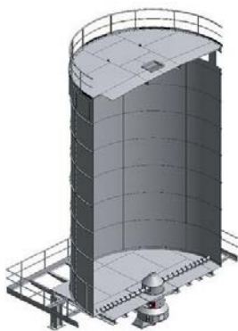
RFU800HD out-feeder mounted in a silo with flat bottom - version with one outlet
